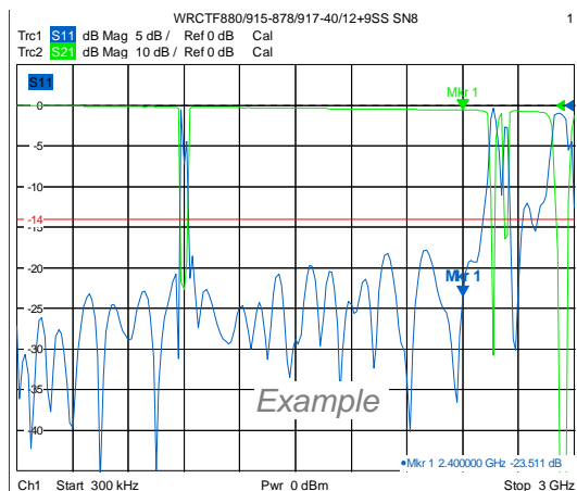
Pass Band Response
