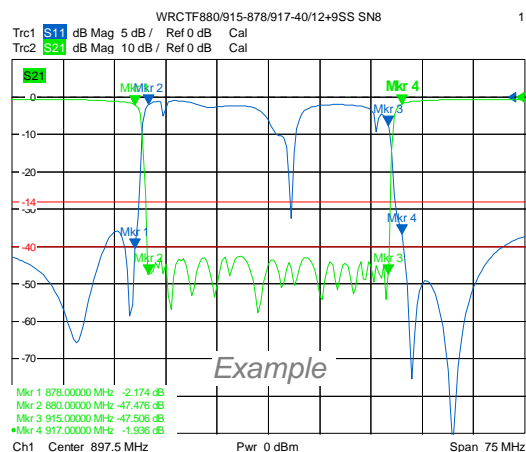
Reject Band Response
