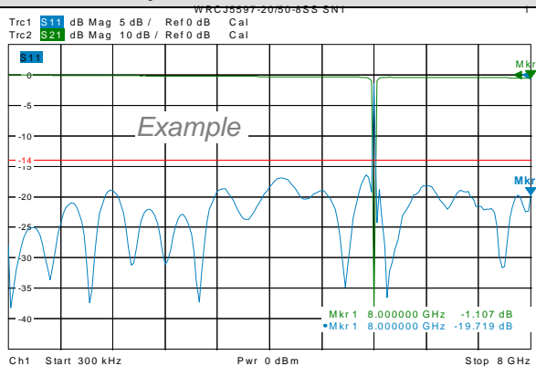
Passband Response
