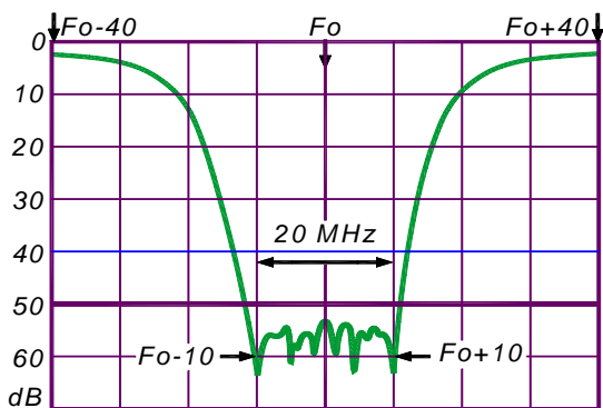
Reject Band Response
