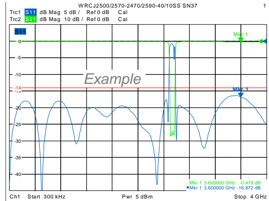
Passband Response
