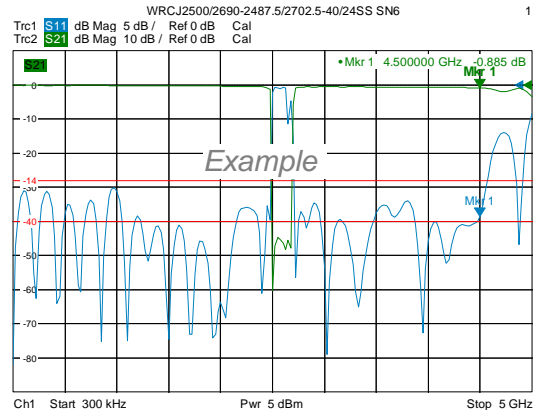
Passband Response
