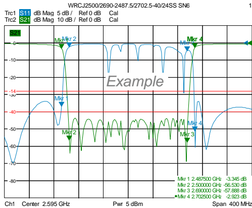
Reject Band Response
