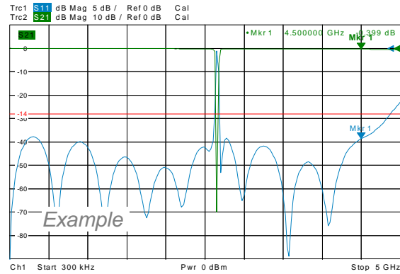
Passband Response
