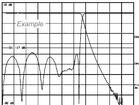
Typical response DC to 1300 MHz
