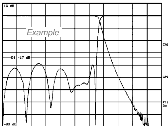
Typical response DC to 1500 MHz
