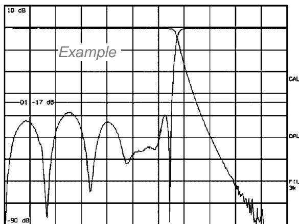
Typical response DC to 1000 MHz
