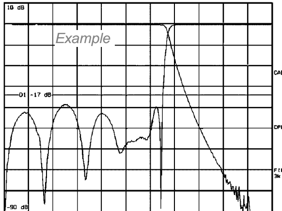
Typical response DC to 700 MHz
