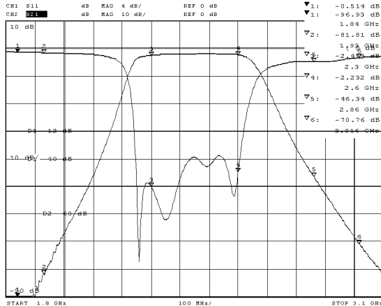
Passband Response
