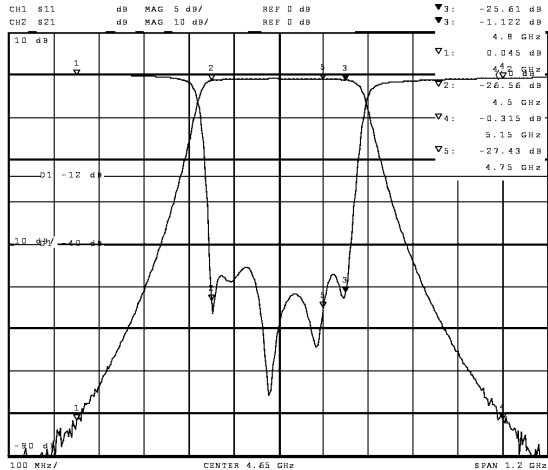
Passband Response
