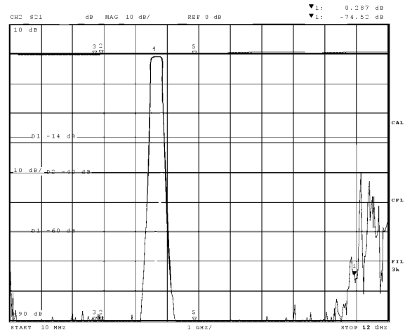
Reject Band Response
