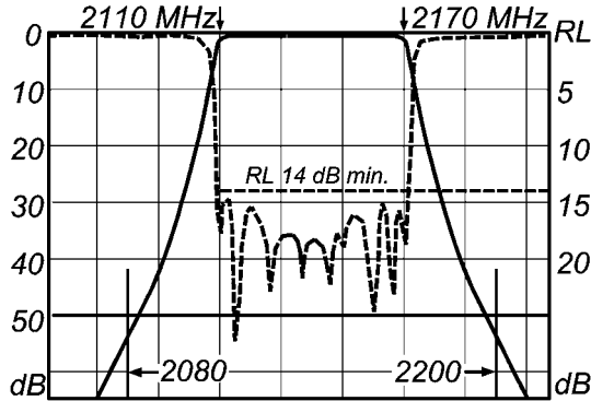
Passband Response
