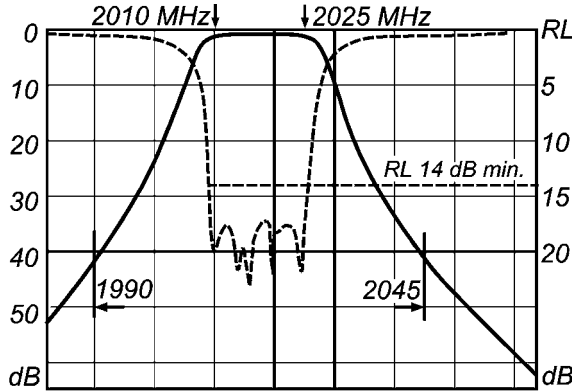
Passband Response
