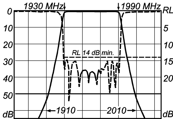
Passband Response
