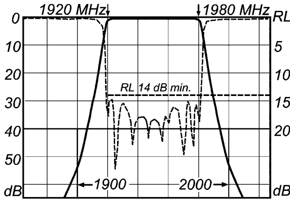
Passband Response
